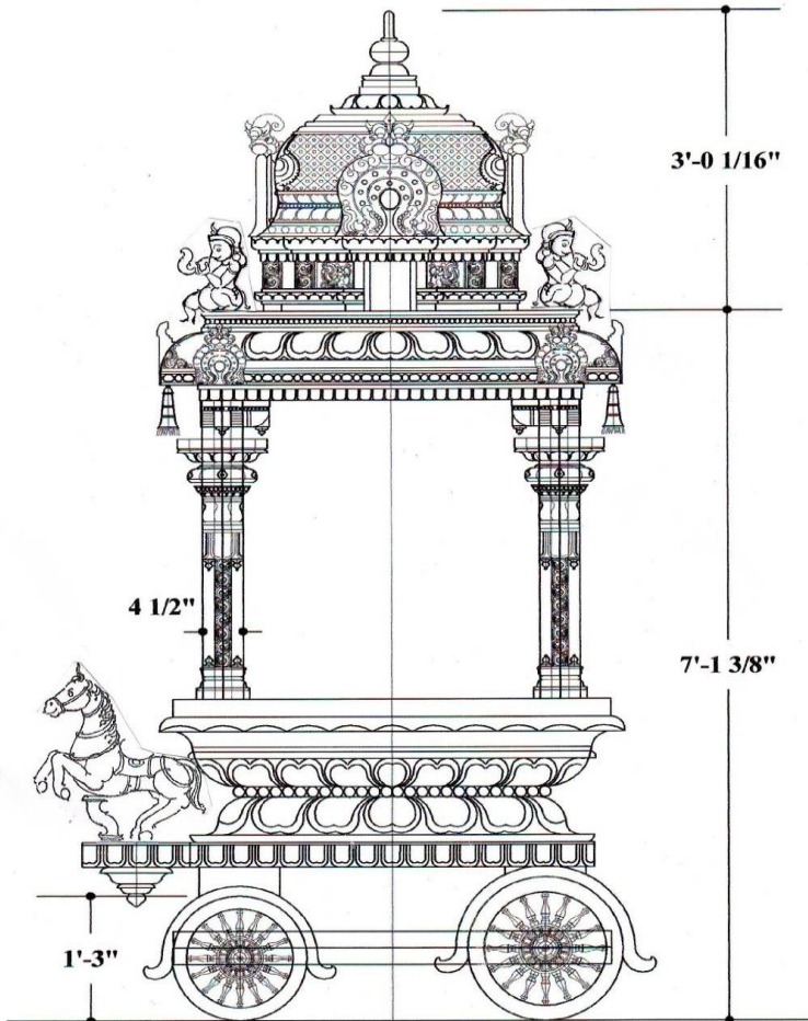
SIDE ELEVATION
